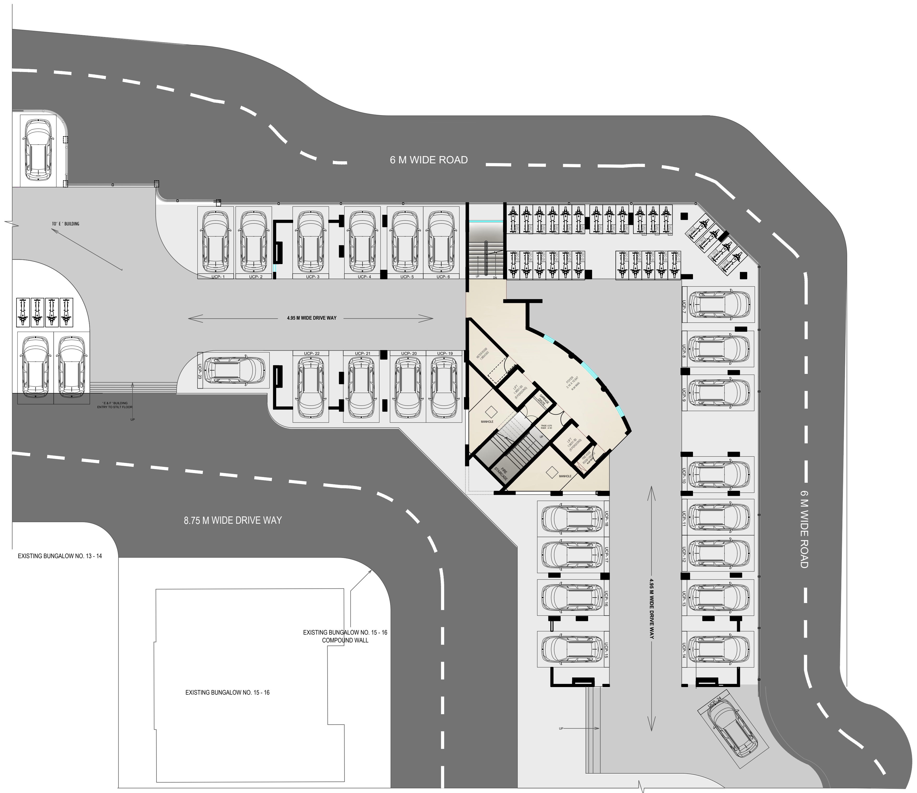
UPPER GROUND FLOOR
